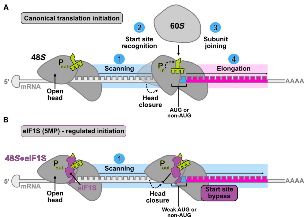
Fig. 6. Schematic of eIF1S (5MP)-mediated regulation of start codon recognition. (A) During canonical initiation, the 48S complex scans the mRNA until it recognizes a start codon. Both canonical AUGs and suboptimal codons, including weak AUGs and non-AUGs, can trigger scanning arrest. This arrest is accompanied by a conformational shift of the 48S head from an open to a closed state, while the initiator tRNA Met transitions from the P out to the P in position to allow codon-anticodon pairing. Successful start site recognition then drives 60S joining and elongation. (B) By contrast, eIF1S (5MP) stabilizes the 48S complex in a scanning-competent state, maintaining the 48S head in the open conformation and the initiator tRNA Met in the P out position. As a result, weak AUG and non-AUG codons fail to induce arrest, are bypassed during scanning, and do not initiate elongation.
