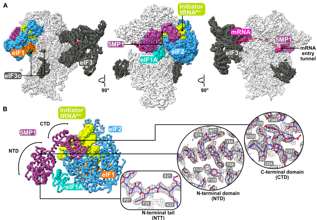
Fig. 3. Cryo-EM of 5MP1 bound to 48S in RRL. (A) A 2.7-Å cryo-EM map of the 48S•5MP1 initiation complex, shown in different orientations. Segmented densities show 5MP1 in purple, eIF2 in blue, eIF1 in orange, eIF1A in turquoise, and the initiator tRNA Met in green. The middle view shows 5MP1 binding at the A site. The left and right show the intersubunit and solvent sides of the 48S initiation complex. (B) 5MP1 interactions with initiation factors and initiator tRNA Met . Insets show the NTT, NTD, and CTD; cryo-EM density is shown as mesh.
