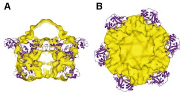
Fig. 7. Comparison of p97/VCP with 20Sm. (A) Side view of 20Sm (yellow) superimposed on the p97/VCP crystal structure (DeLaBarre and Brunger, 2003) (purple). The superposition was carried out by aligning the D1 domain of the p97/VCP structure to the model of the NSF-D1 domain consisting of the NSF-D2 crystal structure fitted to the 20Sm top density in the antiparallel orientation (Figure 5E, right panel). (B) End view of the 20Sm structure. Note the mismatch between the p97/VCP D2 domain with the 20Sm density map (bottom of figure). The orientation of the p97/VCP D2 domain is opposite to that of NSF (compare with Figure 4B).
