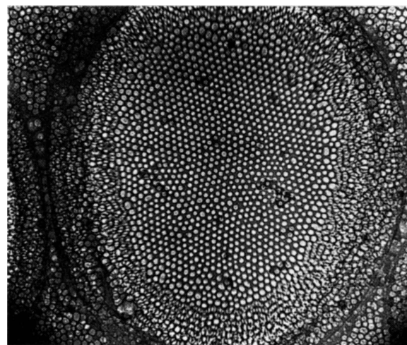
Fig. 1 Electron micrograph of a vitrified sample of 10% F127 solution.
