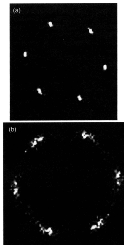
Fig. 4 Diffraction patterns obtained from the Semper analysis: (a) of 10% F127, (b) of 5% F127.
