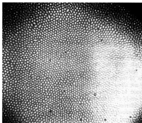
Fig. 2 Electron micrograph of a vitrified sample of 5% F127 solution.
