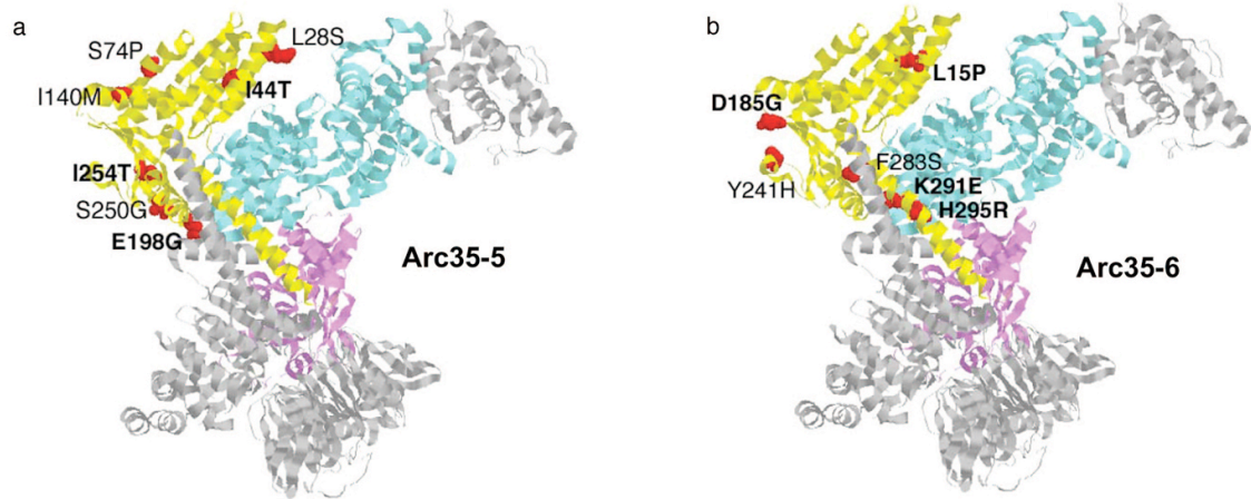
Supplementary Figure 2. Locations of specific mutations in (a) Arc35-5 and (b) Arc35-6 alleles. Residues in the crystal structure of the bovine p34 subunit 1 corresponding to those mutated in yeast Arc35-5 and Arc35-6 are indicated in spacefill. Residues in bold are those that are identical or homologous between yeast and bovine sequences.
