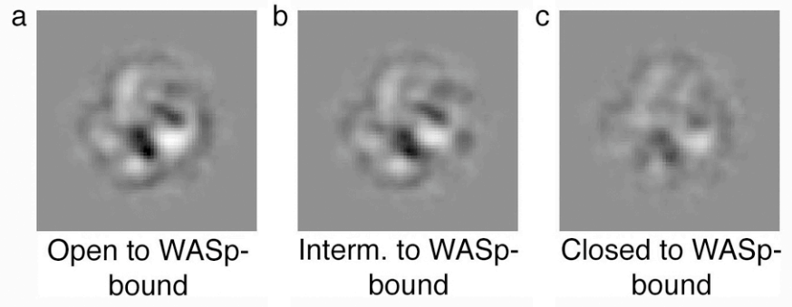
Supplementary Figure 1. Difference maps between WASp-bound Arp2/3 complex and the open ( a ), intermediate ( b ) and closed ( c ) conformations of free complex. The same density scale was used to plot each difference map to emphasize that the difference map in ( c ) contains the smallest peaks.
