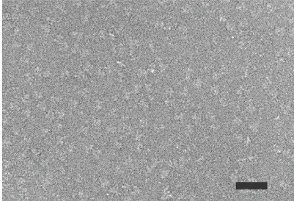
Supplementary Figure 5. Electron micrograph of a field of wild-type Arp2/3 complexes stained with uranyl formate. Scale bar is 200 Å.
