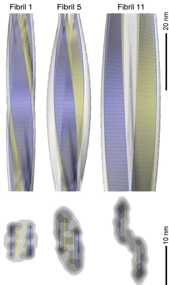
Fig. 6. Structural model of the protofilament core topology of fibrils 1, 5 and 11. Top, side view of the fibrils with two protofilament cores modeled into the densities. Bottom, contoured density cross-sections of the fibrils superimposed with two protofilament cores. Each protofilament core comprises a pair of two \beta -sheet regions colored in yellow (interface) and blue (outside). Each \beta -sheet region may be formed by one A \beta peptide, as suggested by a recent analysis of a morphology corresponding to fibril 11. 36 To date, it is not known whether a \beta -sheet region consists of a single long strand or whether it is constructed from several short \beta -sheet segments.
