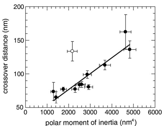
Fig. 5. Correlation between crossover distance ( d ) and polar moment of inertia ( I_2 ). The data are given in Table 1. Filled circles represent fibrils 1–11, open circle represents fibril 12. Only the data points of fibrils 1–11 are fit with a straight line ( R = 0.93 ).
