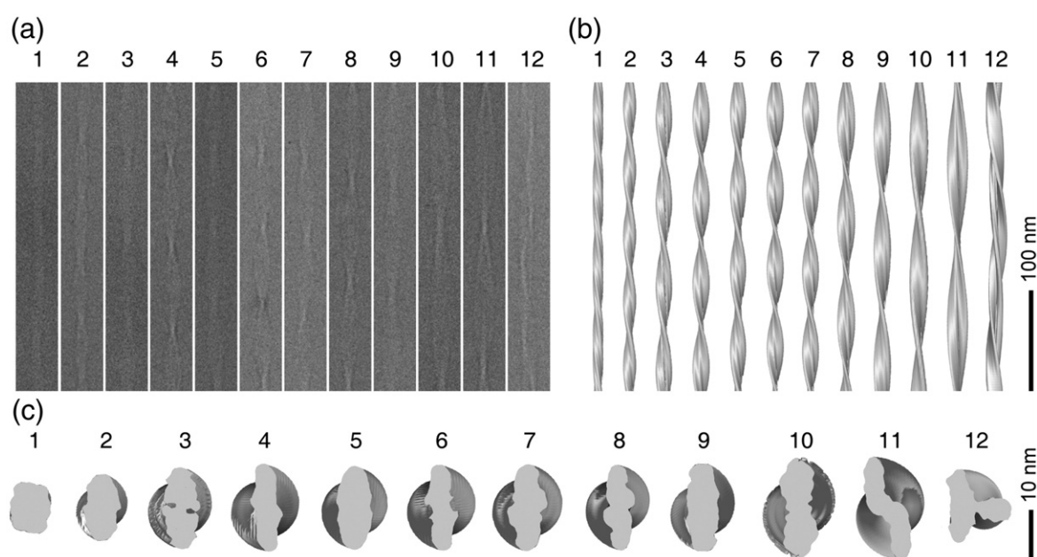
Fig. 2. Cryo-EM reconstructions of 12 individual A \beta (1-40) fibrils. (a) Electron micrographs of the 12 individual A \beta (1-40) fibrils from the same sample. (b and c) Side (b) and top (c) views of the reconstructed fibrils shown in (a).
