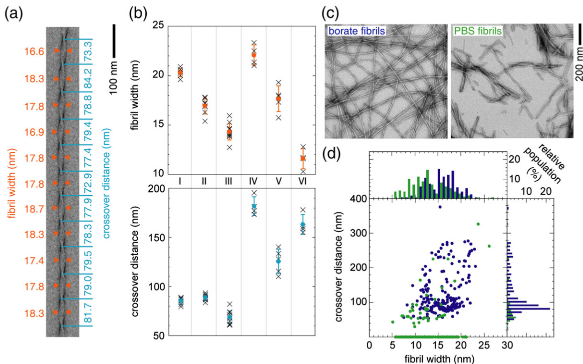
Fig. 1. Demonstration of the structural persistence and morphological diversity of A \beta (1-40) fibrils. (a) Example measurement of fibril width and crossover distance at different positions on the same fibril. (b) Plot of fibril width and crossover distance measured for six different fibrils grown in 50 mM sodium borate (pH 7.8) at 22 °C. Columns I–VI show the values measured at different positions of the same fibril (crosses) and their mean with standard deviation (filled circles). (c) Negative stain images of A \beta (1-40) fibrils grown either in 50 mM sodium borate (pH 7.8) at 22 °C or in PBS (pH 7.4) at 37 °C. (d) Distribution of fibril width ( w ) and crossover distance ( d ) of different individual fibrils formed in sodium borate buffer (black) or PBS (gray). Data points with d = 0 represent fibrils with no measurable d value (see the text for details).
